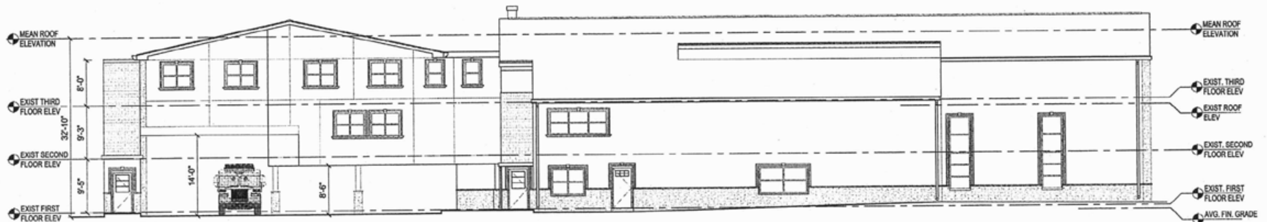
SOUTH ELEVATION
