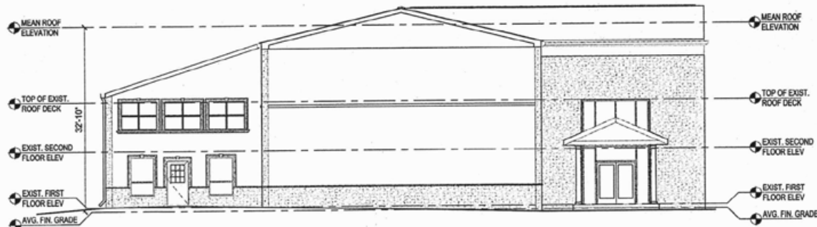
EAST ELEVATION
